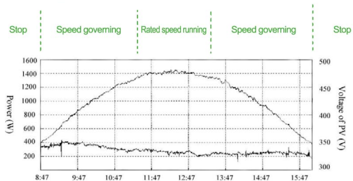
Daily operation curve on a sunny day
